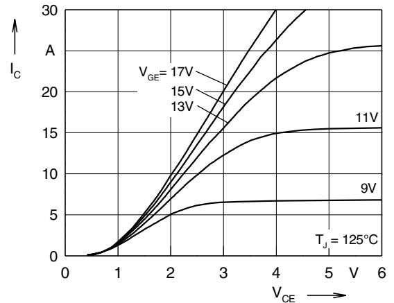
Fig. 8 Typ. output characteristics
